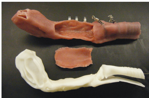
3D printed components were used in a prototype airway trainer
